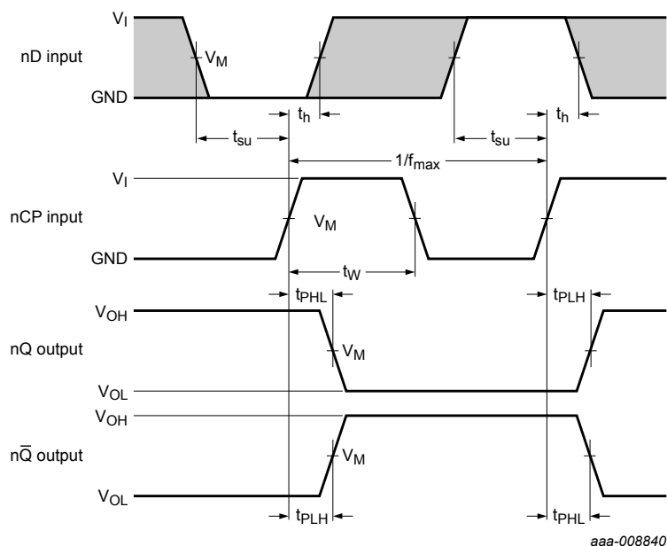
Figure 8. Clock pulse (nCP) to output (nQ, nQ̄) propagation delays, nCP pulse width, the nD to nCP set-up times, the nCP to nD hold times and maximum frequency
